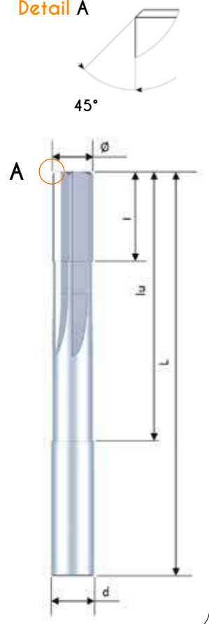
Detail A
